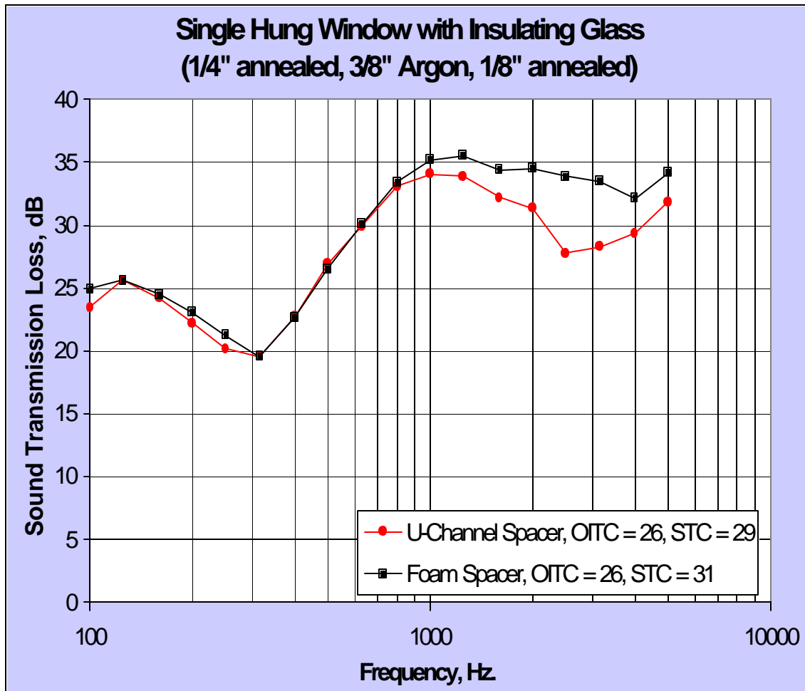
Figure 3.7 - Spacer Effect on Sound Transmission Loss
