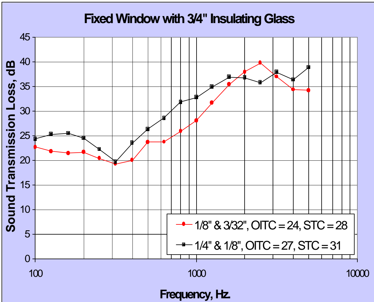
Figure 3.1 - Glass thickness (mass) effect on sound transmission loss
