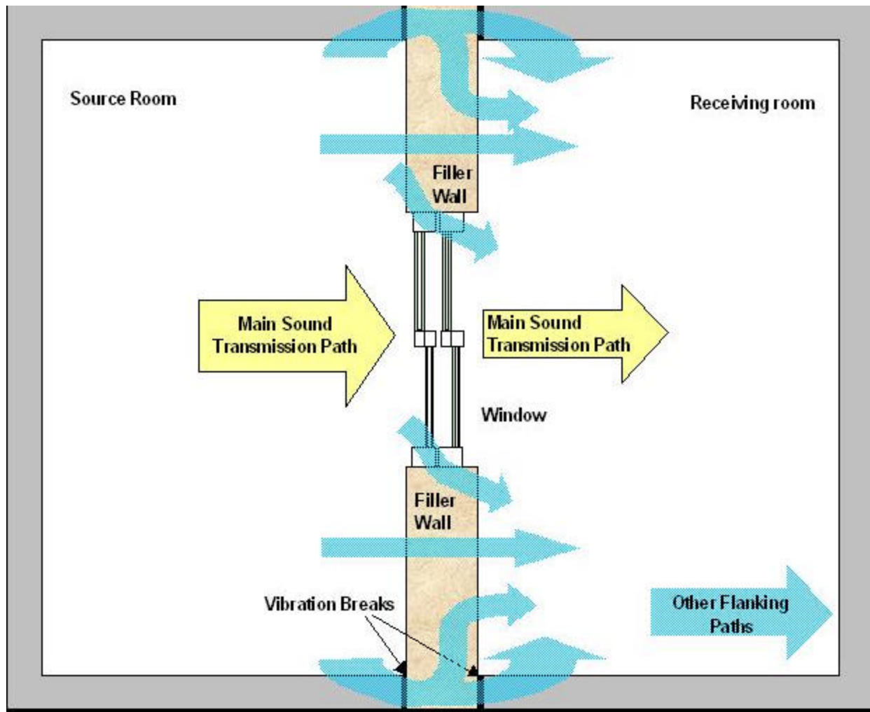
Figure 1.7.1 - Flanking Effects on Sound Transmission Loss in the Laboratory
