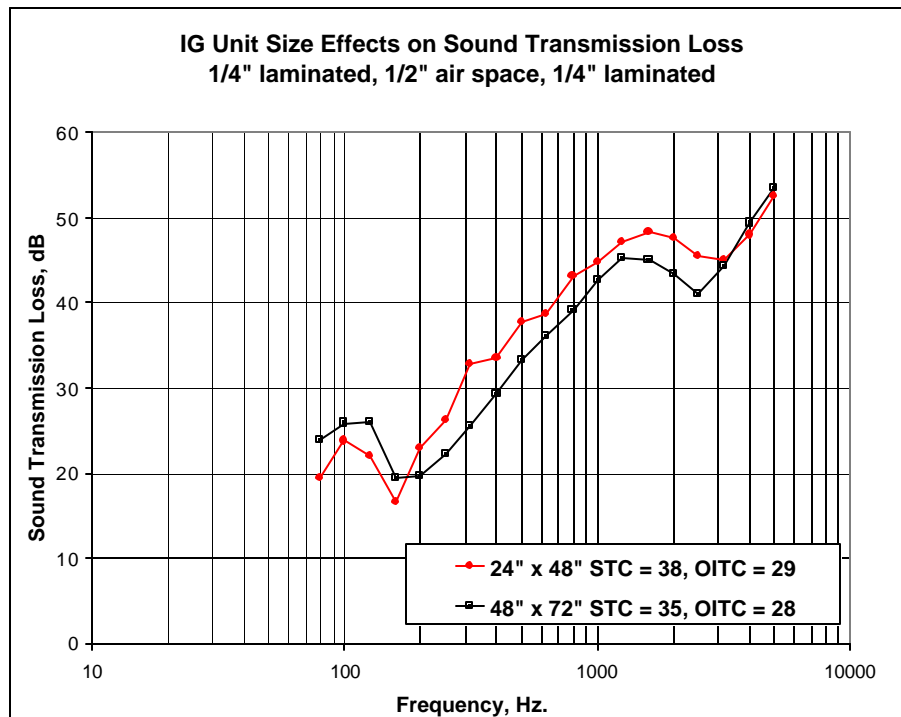
Figure 3.9.1 - Glass Size Effect for Annealed Glass
