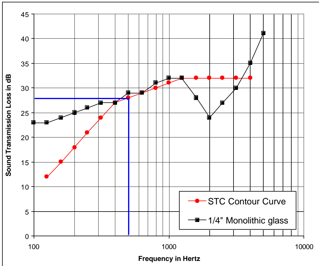
Figure A1.1 - Typical STC Contour (STC-28).
