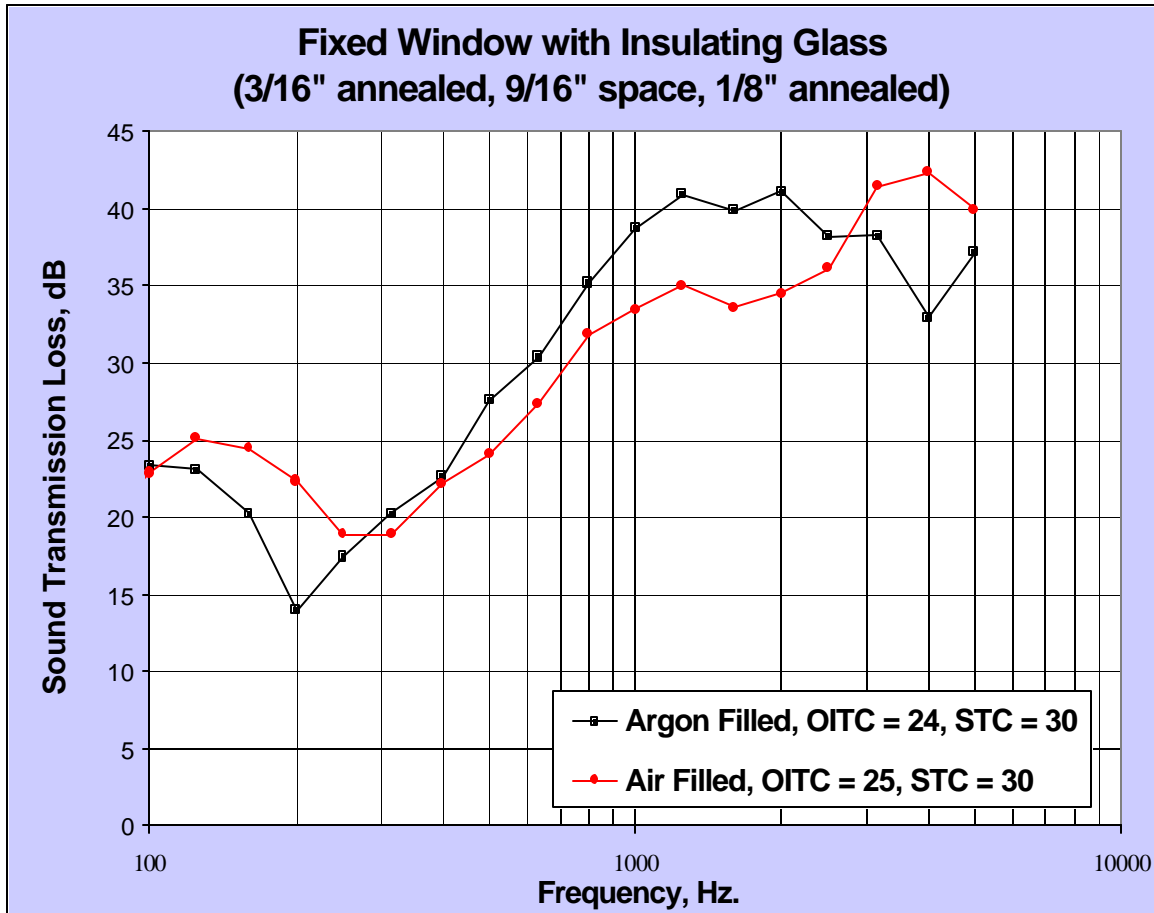
Figure 3.6 - Gas fill effect sound transmission loss
