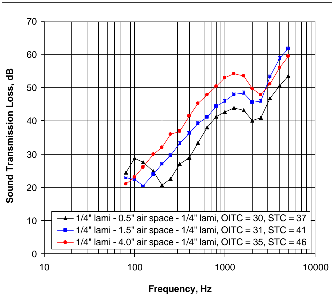
Figure 1.6.2 - Shift in Mass-Air-Mass Resonance with Larger Air Spaces
