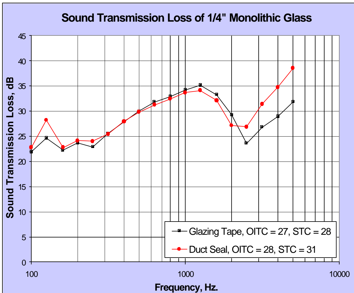
Figure 3.8 - Edge Damping Effect on Glass Panels
