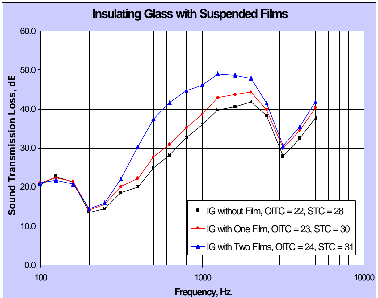
Figure 3.5 - Suspended films in insulating glass units
