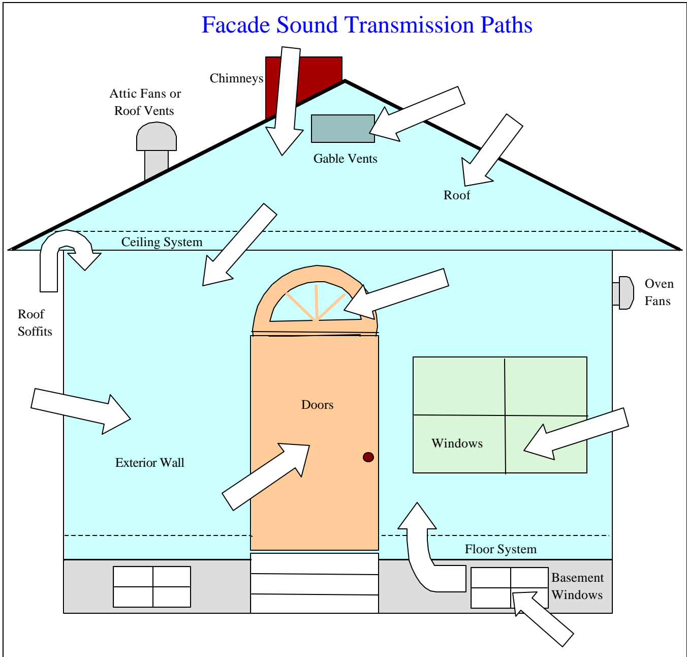
Figure 1.7.2 Residential Flanking Problems
