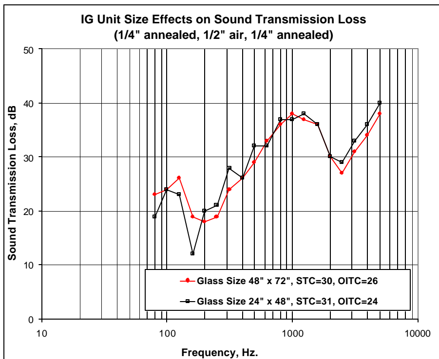
Figure 3.9.2 - Glass Size Effect for Laminated Glass
