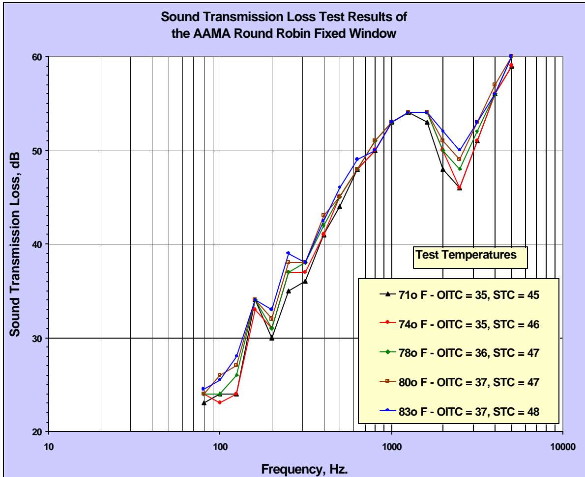
Figure 3.3 - Temperature effect on laminated glass
