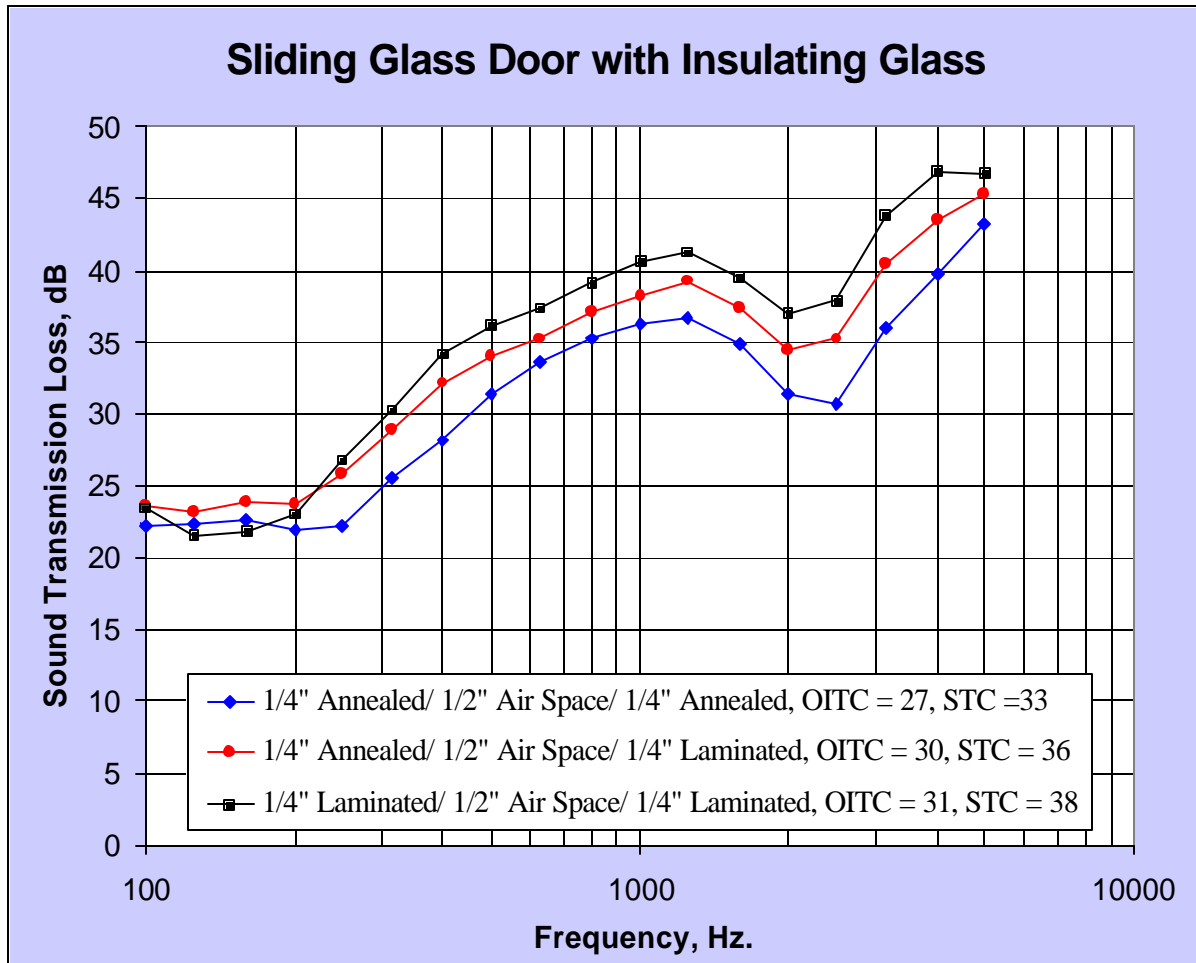
Figure 3.2 - Annealed versus laminated glass performance
