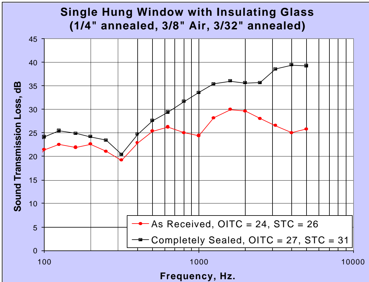
Figure 4.1 - Air Leakage Effect on Sound Transmission Loss
