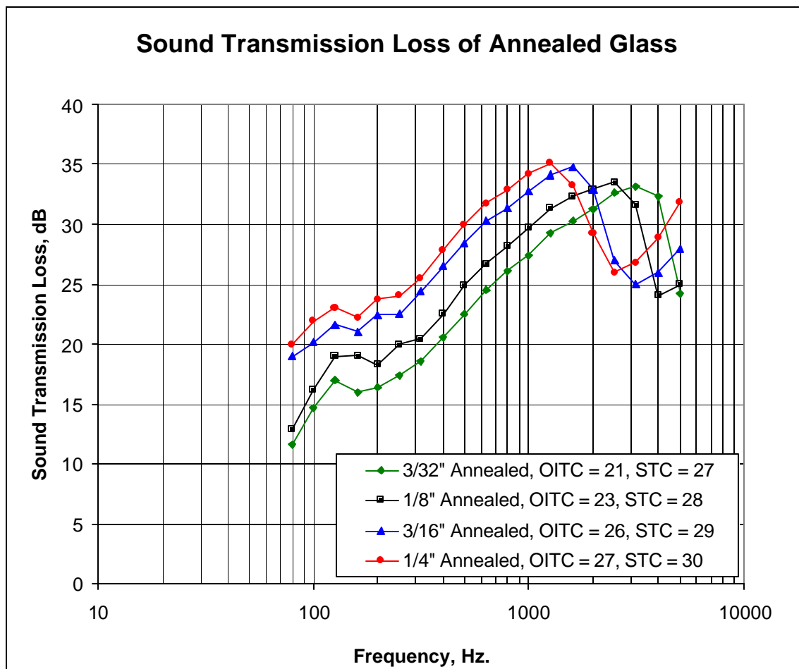
Figure 1.6.1 - Coincidence Dip for Various Glass Thickness
