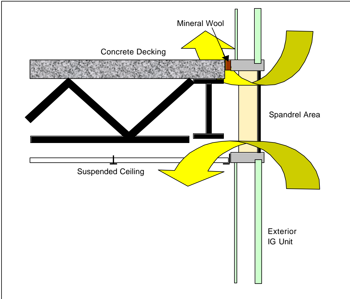
Figure 1.7.3 - Flanking Paths for a Curtain Wall Assembly
