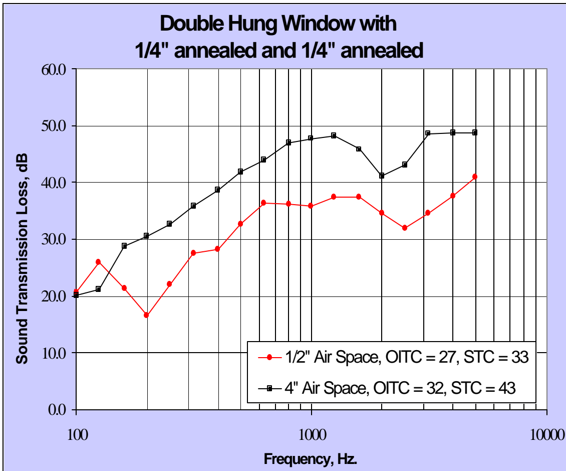
Figure 3.4 - Air Space Effect on Sound Transmission Loss
