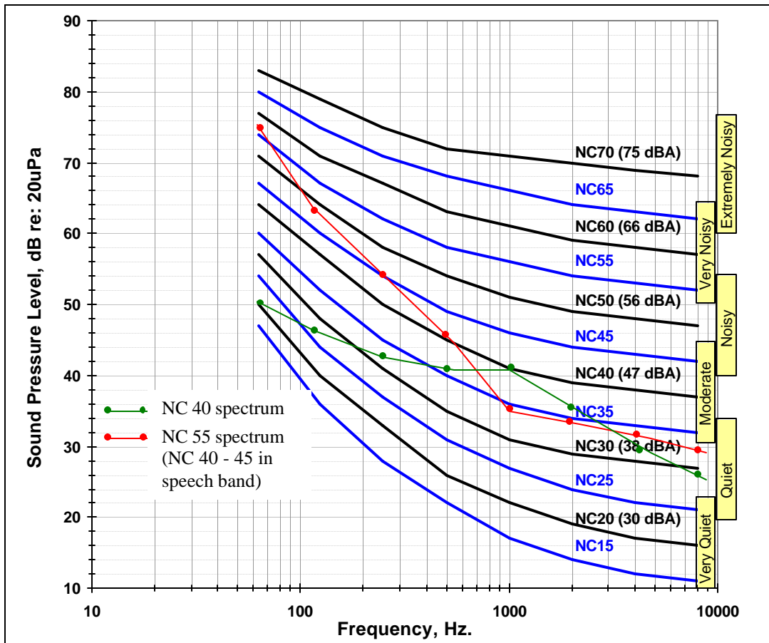
Figure 1.11 - Noise Criteria Curves
